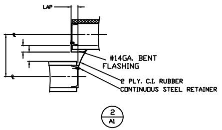
TYPICAL HANGAR DOOR SEALS
