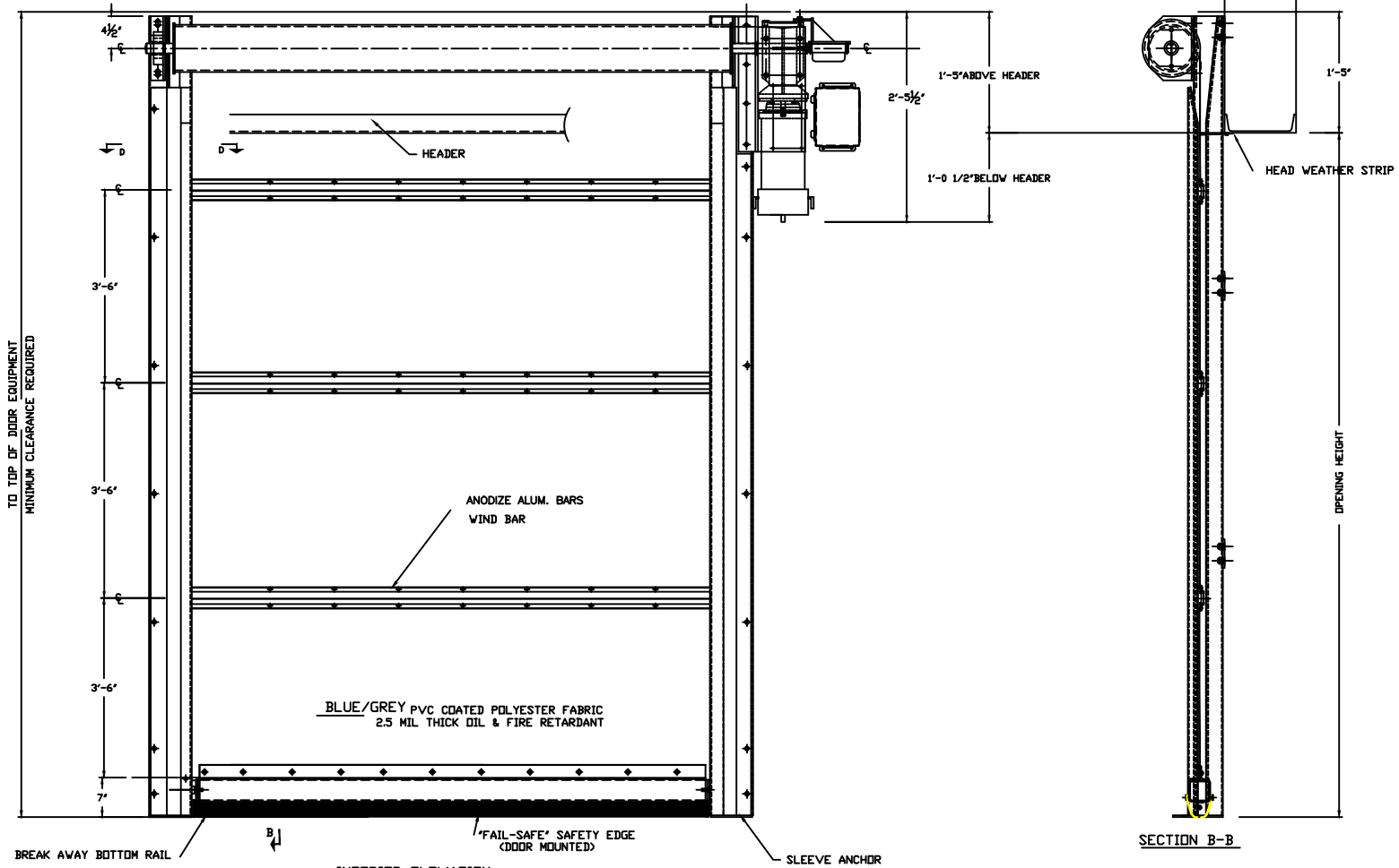
INTERIOR ELEVATION HIGH SPEED ROLLING FABRIC DOOR- *U.S JET DOOR -MODEL 2004-A
